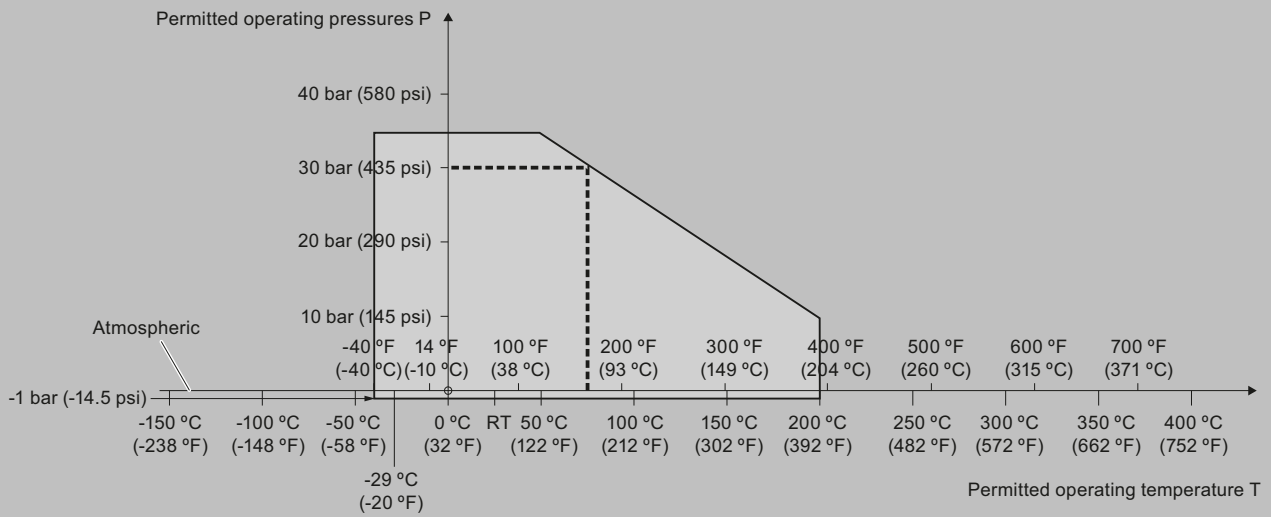
Pointek CLS300 process pressure/temperature derating curves (7ML5650, 7ML5651, 7ML5660, and 7ML5661 )
