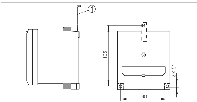
Fig. 5: Screw mounting
