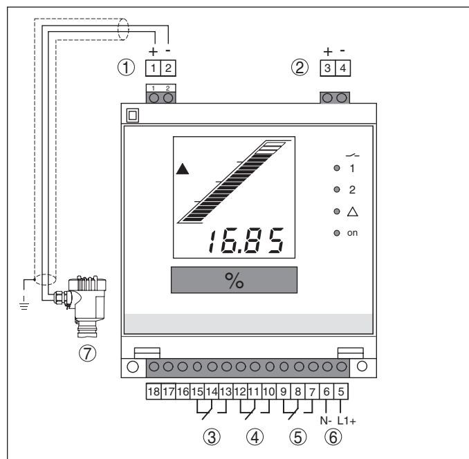
Fig. 11: Wiring plan with two-wire sensor
