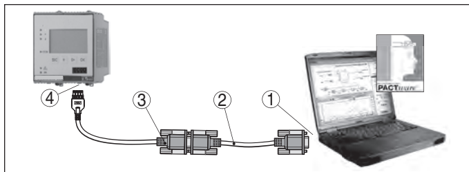
Fig. 23: Connection of the PC via RS232
