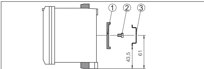
Fig. 6: Carrier rail mounting
