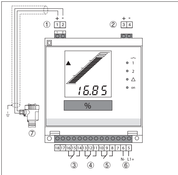
Fig. 12: Wiring plan with two-wire sensor
