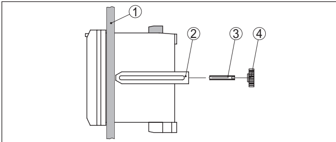
Fig. 4: Front panel mounting
